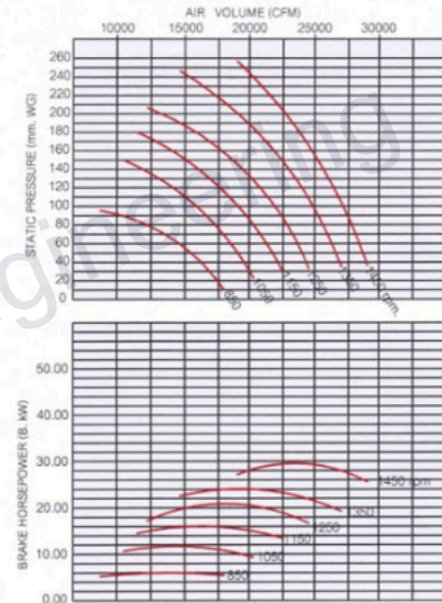
CENTRIFUGAL FAN 36" (BACKWARD CURVED BLADE)
