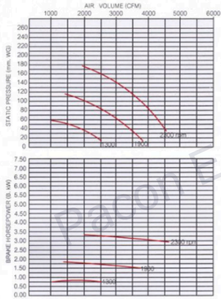
CENTRIFUGAL FAN 30" (BACKWARD CURVED BLADE)
