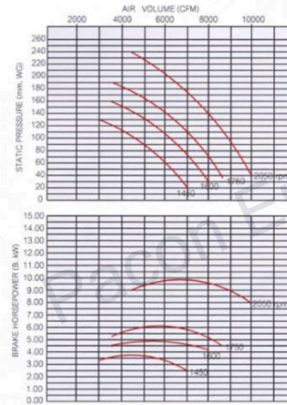
CENTRIFUGAL FAN 24" (BACKWARD CURVED BLADE)
