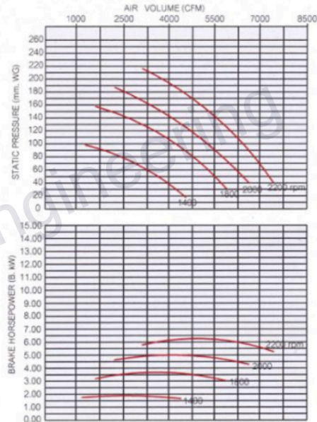
CENTRIFUGAL FAN 36" (BACKWARD CURVED BLADE)
