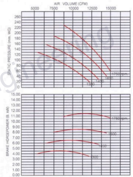
CENTRIFUGAL FAN 27" (BACKWARD CURVED BLADE)
