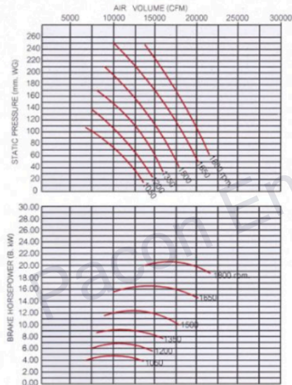
CENTRIFUGAL FAN 30" (BACKWARD CURVED BLADE)
